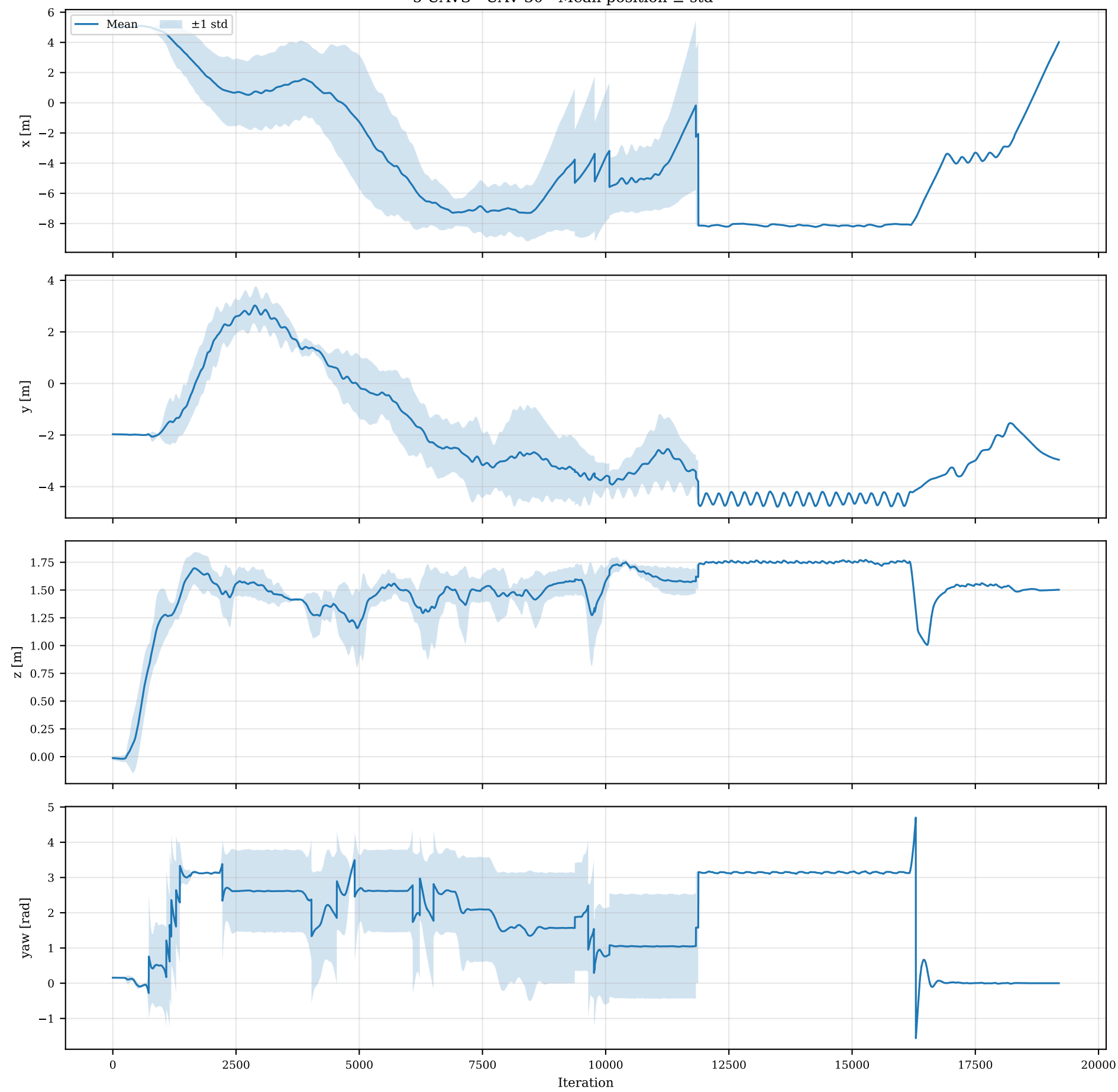
5 UAVS - UAV 30 - Mean position \pm std
